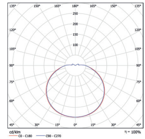
45 W/830, 4600 lm netto
